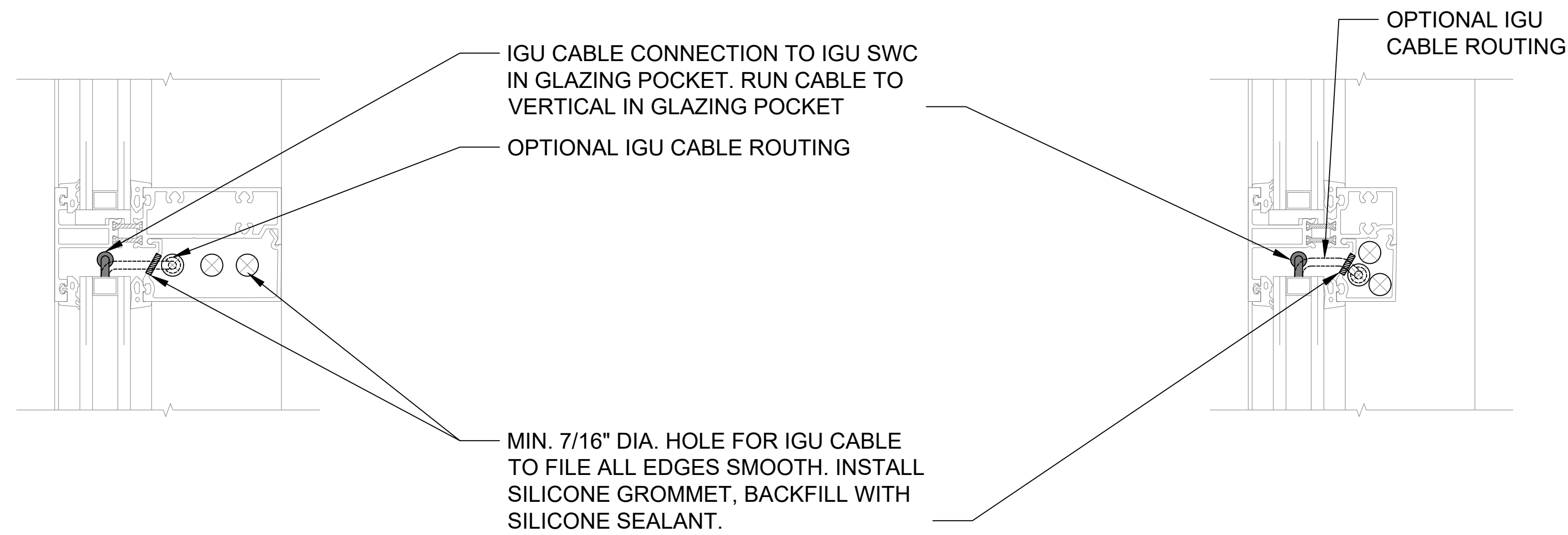
DETAIL 2 HORIZONTAL MULLION
